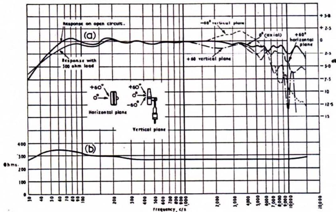
Fig. 19 — Microphone Type PGS
