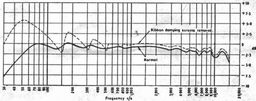
Fig. 7 — Microphone Type PGS. Open-circuit axial frequency response with and without ribbon damping screens
