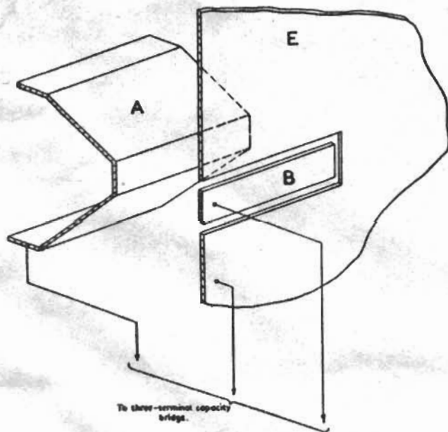
Fig. 5 — Microphone Type PGS. Section of Electrostatic model used for determination of Magnetic Leakage (Simplified Diagram)
