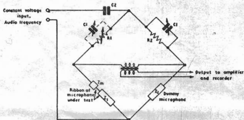
Fig. 9 — Motional impedance bridge circuit
