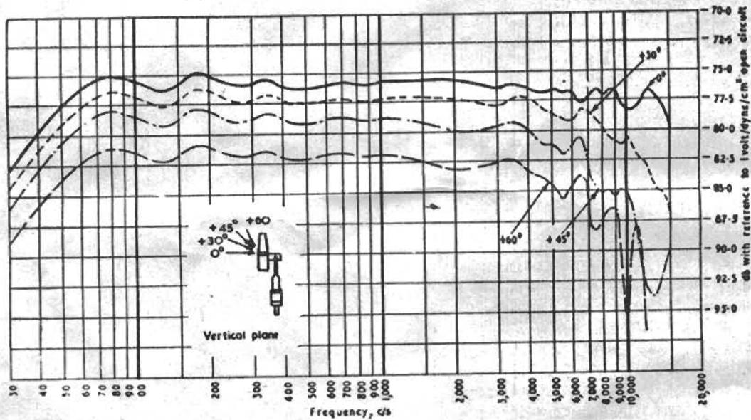
Fig. 17 — Microphone Type PGS. Open-circuit frequency response in vertical plane above axis
