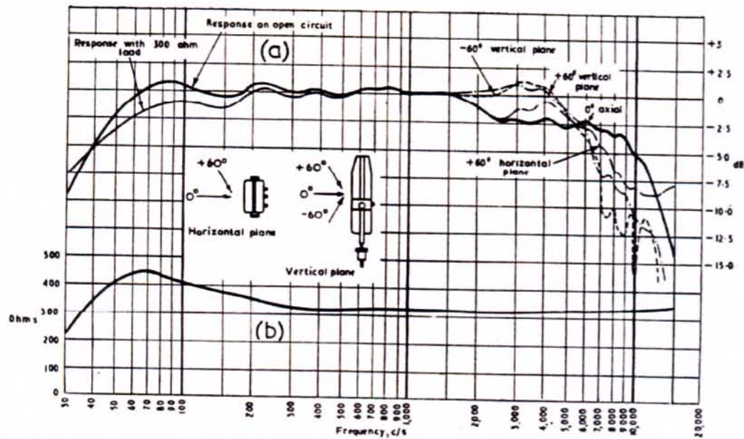
Fig. 20 — Microphone Type PGD
