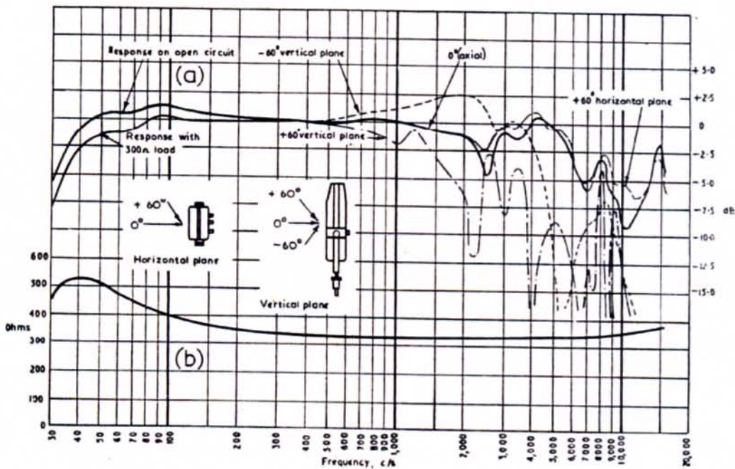
Fig. 21 — Microphone Type AXBT
