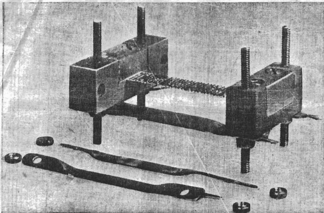
Fig. 14 — Microphone Type PGS. Ribbon carrier with ribbon
