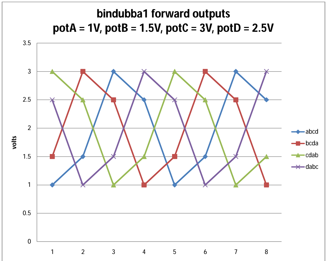
Figure 2: forward counting output voltages for 8 clock pulses
