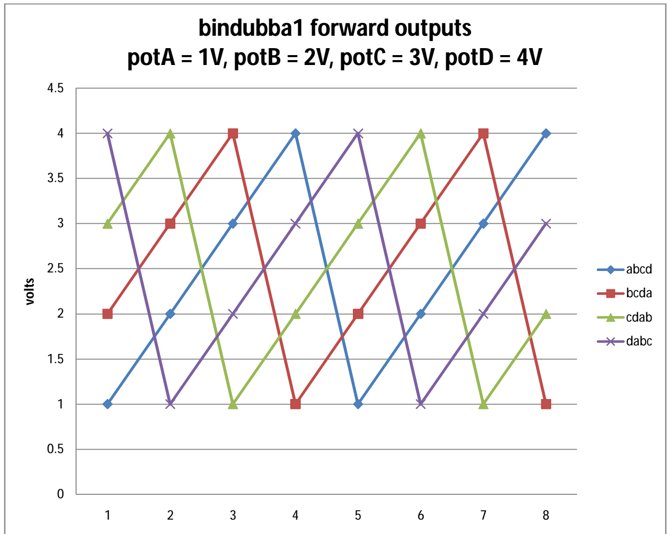
Figure 1: forward counting output voltages for 8 clock pulses
